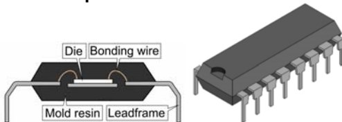
DIP Examples
