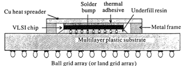
Lidded BGA Cross Section
